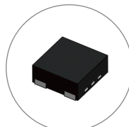
DFN2020-6(SD) 2.0*2.0*0.6
